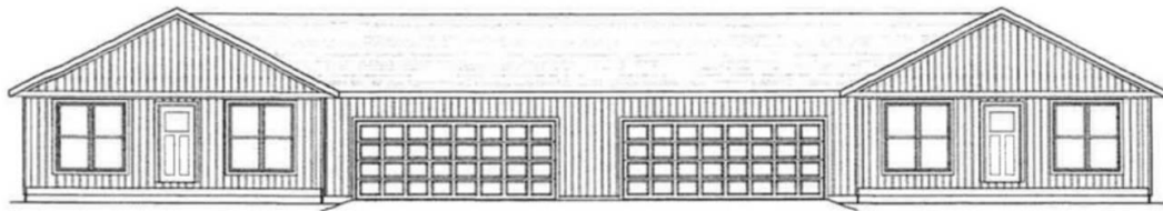
FRONT ELEVATION 1/4" = 1'-0"
