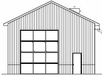
3 FRONT ELEVATION SCALE 1/8" = 1'-0"
