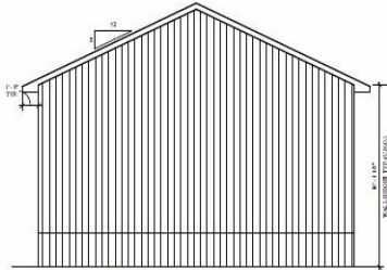
2 BACK ELEVATION SCALE 1/8" = 1'-0"
