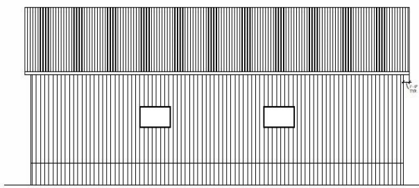
1 RIGHT ELEVATION SCALE 1/8" = 1'-0"
