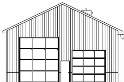
3 FRONT ELEVATION SCALE 1/8" = 1'-0"
